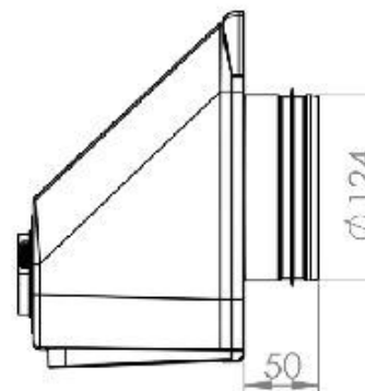
VILPE® IO 125 wall element
